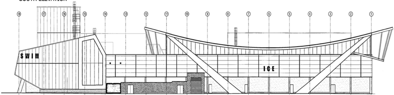
EAST ELEVATION
