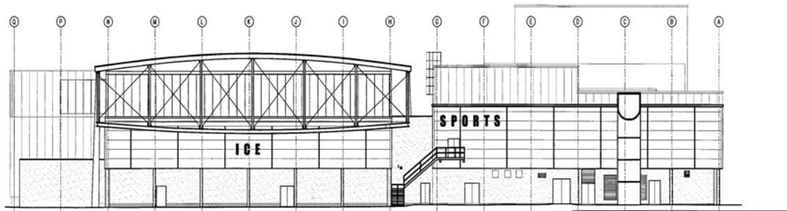
NORTH ELEVATION
